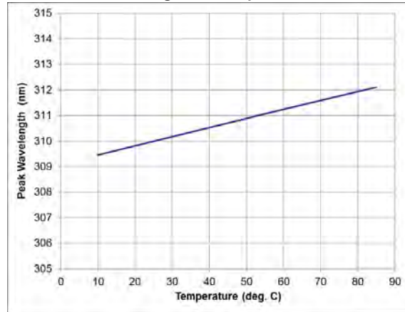
Peak Wavelength vs. Temperature 310nm
